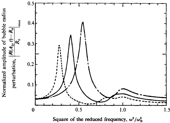
FIGURE 8. Normalized amplitude of the bubble-radius damped oscillations at the cloud surface ( r = A_0 ) as a function of the squared reduced frequency \omega^2/\omega_B^2 at various void fractions. The curves refer to the following values of the parameter 3\alpha_0(1-\alpha_0)A_0^2/R_0^2 : \frac{1}{4}\pi^2 (solid line); \frac{1}{8}\pi^2 (dash-dotted line); and \frac{1}{2}\pi^2 (dotted line).
