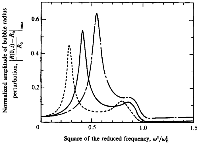
FIGURE 12. Normalized amplitude of the bubble-radius damped oscillations at the cloud centre ( r = 0 ) as a function of the squared reduced frequency \omega^2/\omega_B^2 at various void fractions. Notation as figure 8.
